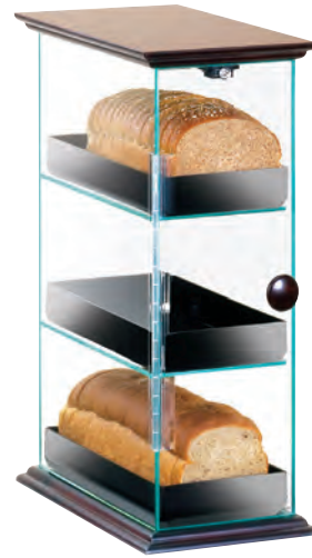
1204-52
